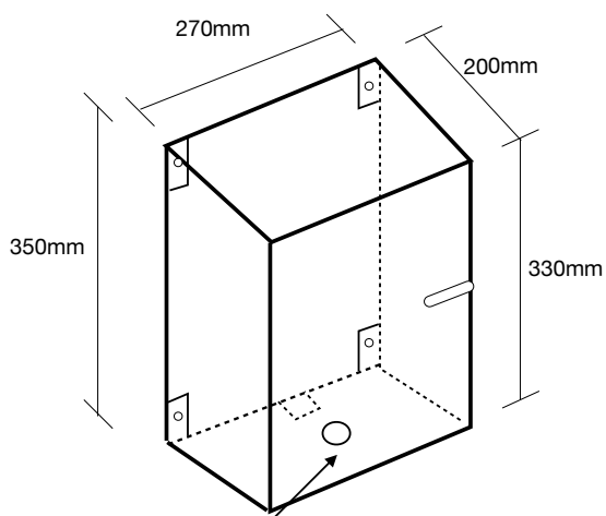
25mm Hole with rubber grommet Set at 80mm centre from the front of the box.
